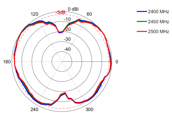
Elevation: 2400 - 2500 MHz
