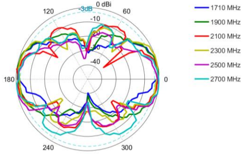
Elevation: 1710 – 2700 MHz
