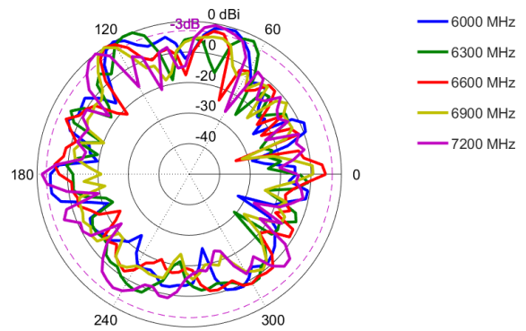
Elevation: 6000 – 7200 MHz
