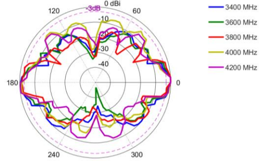
Elevation: 3400 – 4200 MHz
