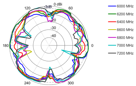
Elevation: 6000 - 7200 MHz
