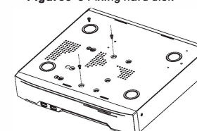
Figure3-3 Fixing hard disk
