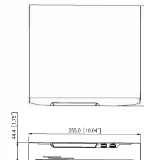
Figure 2-1 Dimensions (Unit:mm)
